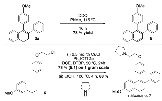
Scheme 2. Intermolecular Carboarylation
